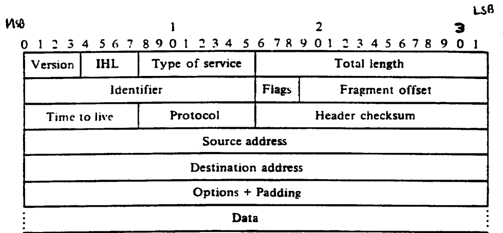
generic IP packet (IPv4)
